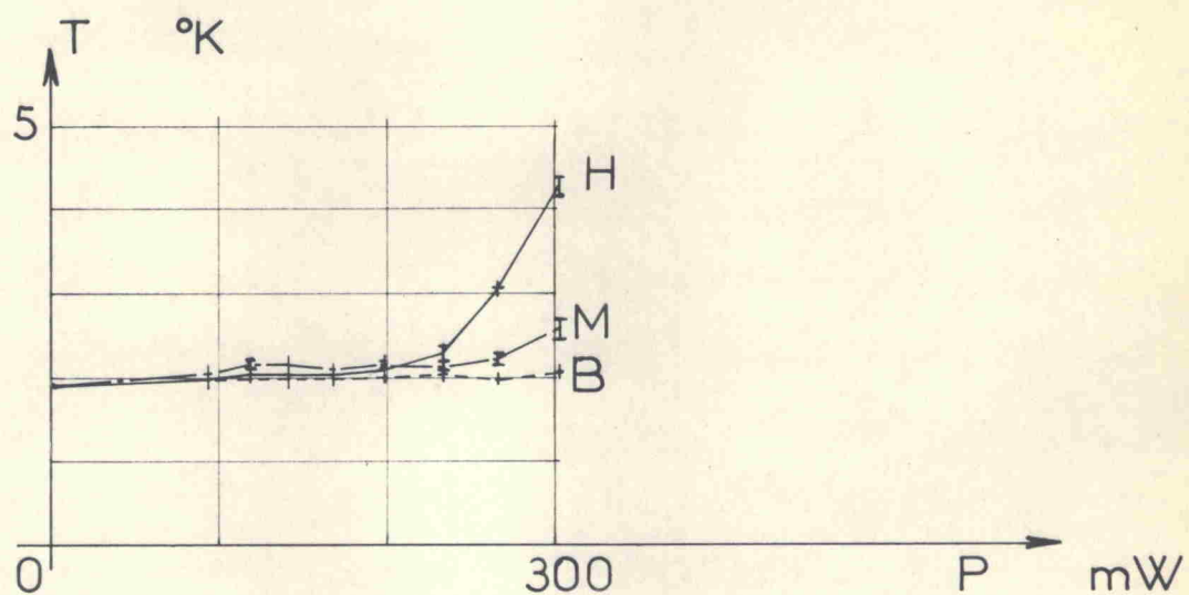
FIG. 3 : Superfluid helium T = 1.9 K; P = 17.6 mm Hg Depth of immersion : 20 cm
