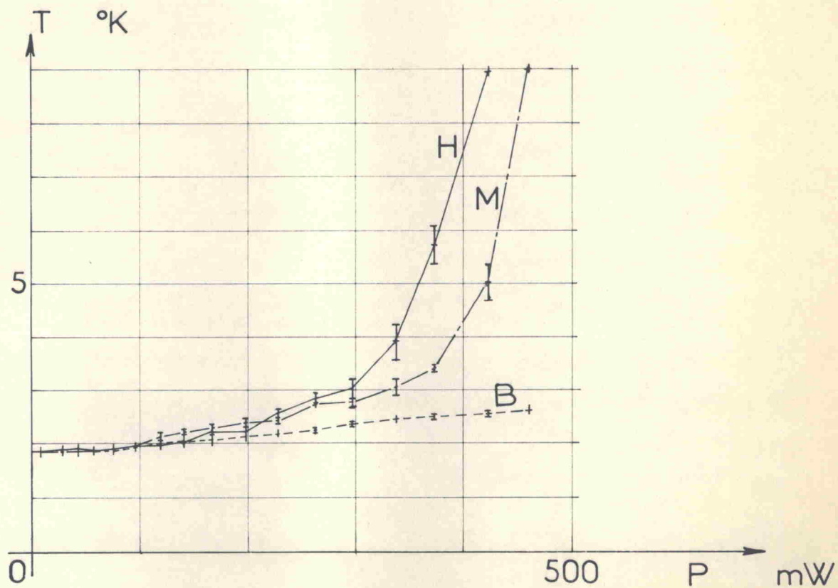
FIG. 4 : Unsaturated superfluid helium T = 1.85 K ; P = 32.5 mm Hg
